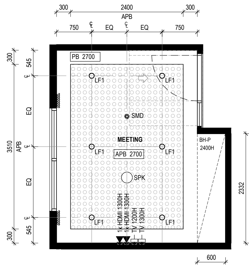
2 RCP - VILLAGE ADMIN - MEETING Scale 1 : 50
