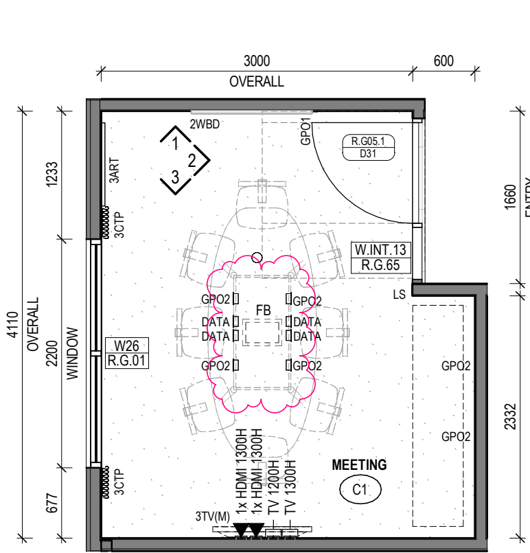
1 VILLAGE ADMIN - MEETING Scale 1 : 50
