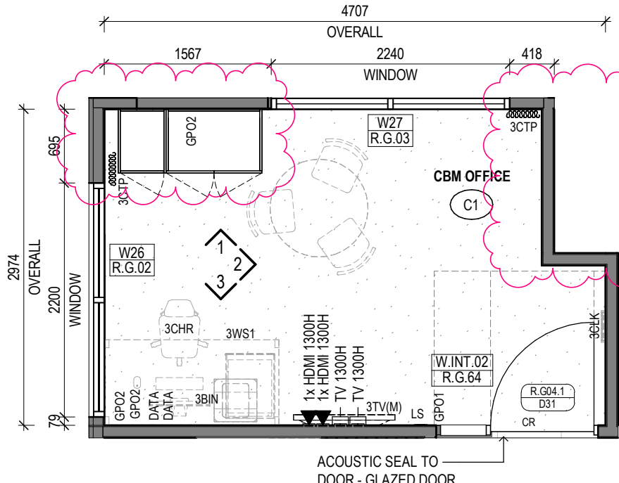
3 VILLAGE ADMIN - CBM OFFICE Scale 1 : 50
