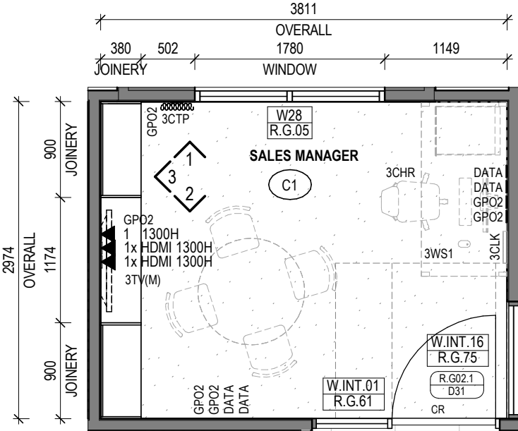
5 VILLAGE ADMIN - SALES MANAGER Scale 1 : 50
