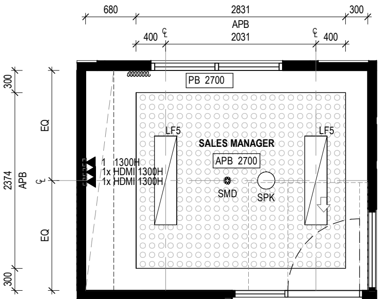
6 RCP - VILLAGE ADMIN - SALES MANAGER Scale 1 : 50
